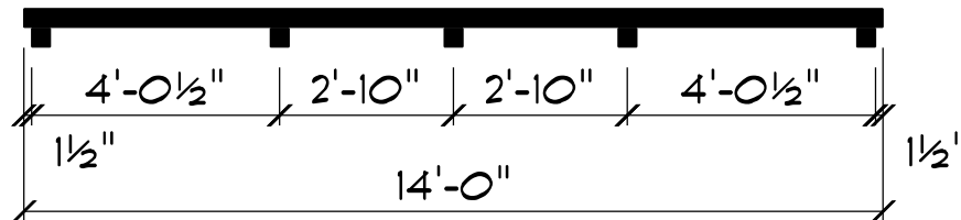
14' Wide Building
