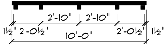
10' Wide Building
