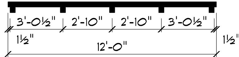
12' Wide Building
